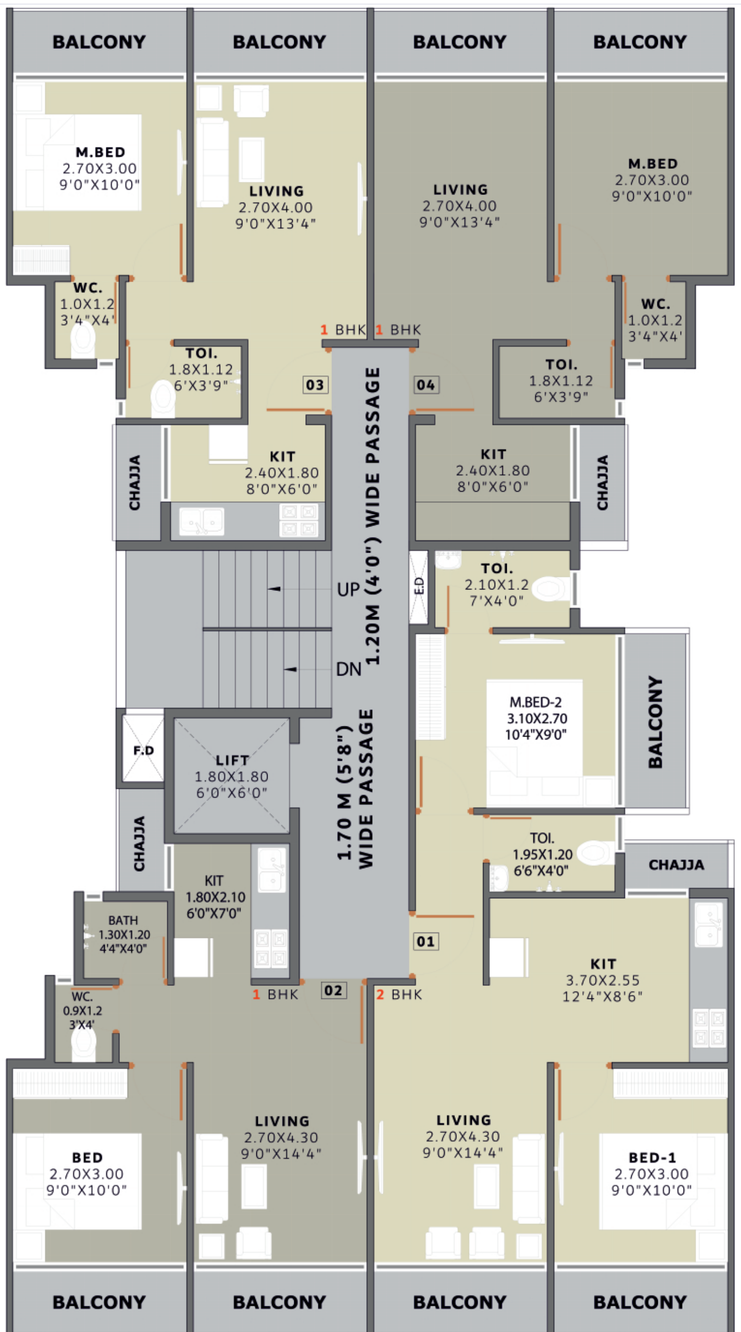
TYPICAL FLOOR PLAN
